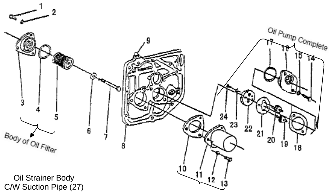
Fig. 9. Lubricating System
