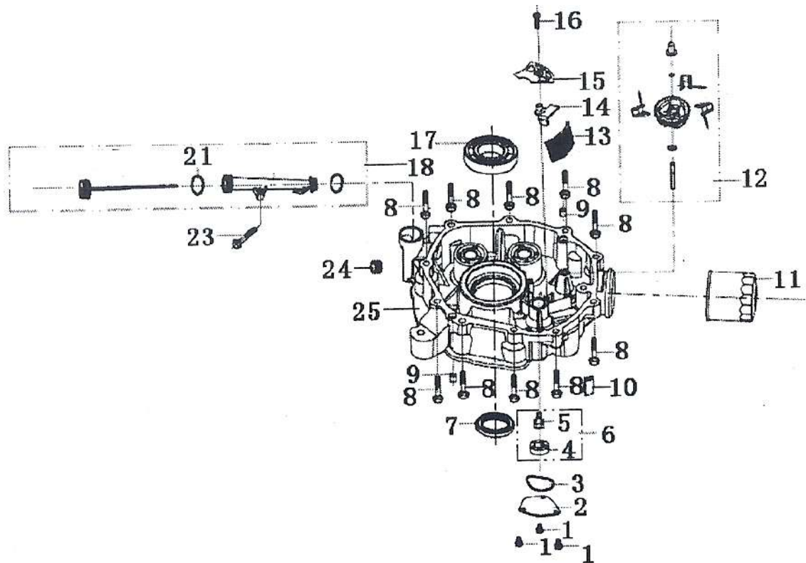
CRANKSHAFT COVER
