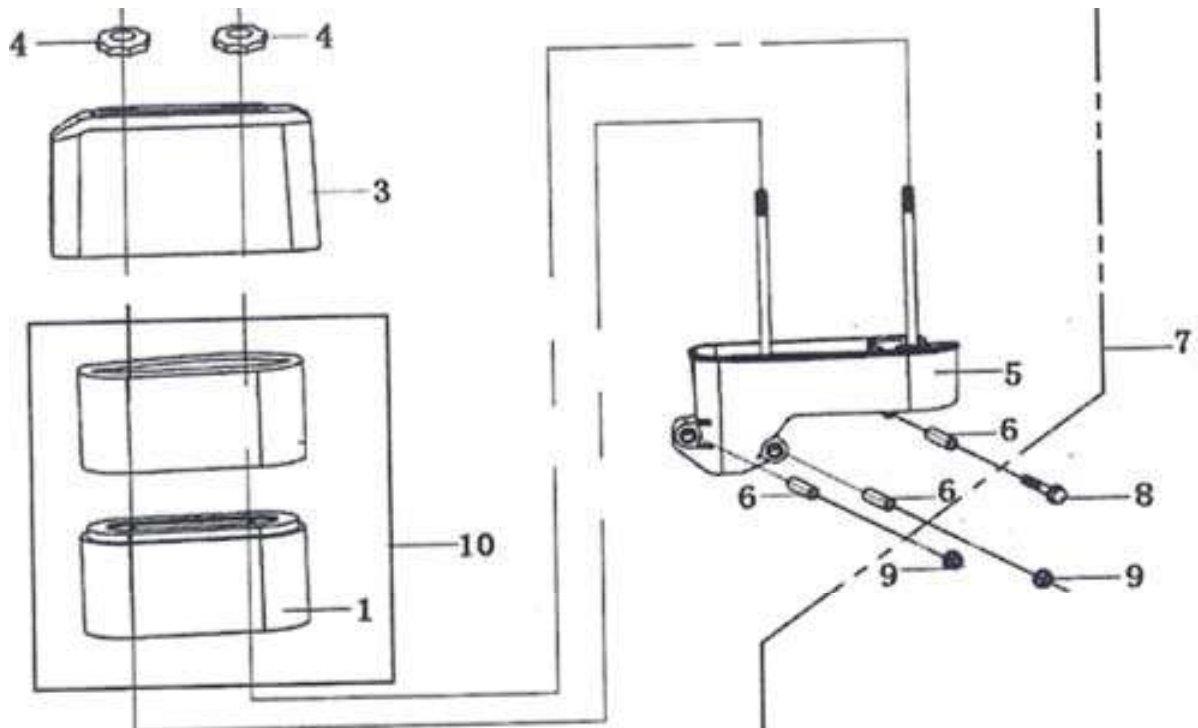
AIR CLEANER
