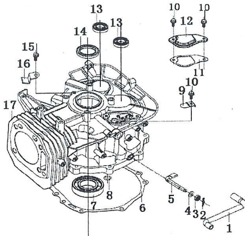
CRANKCASE
