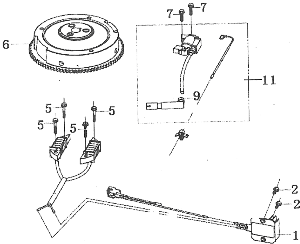
FLYWHEEL
