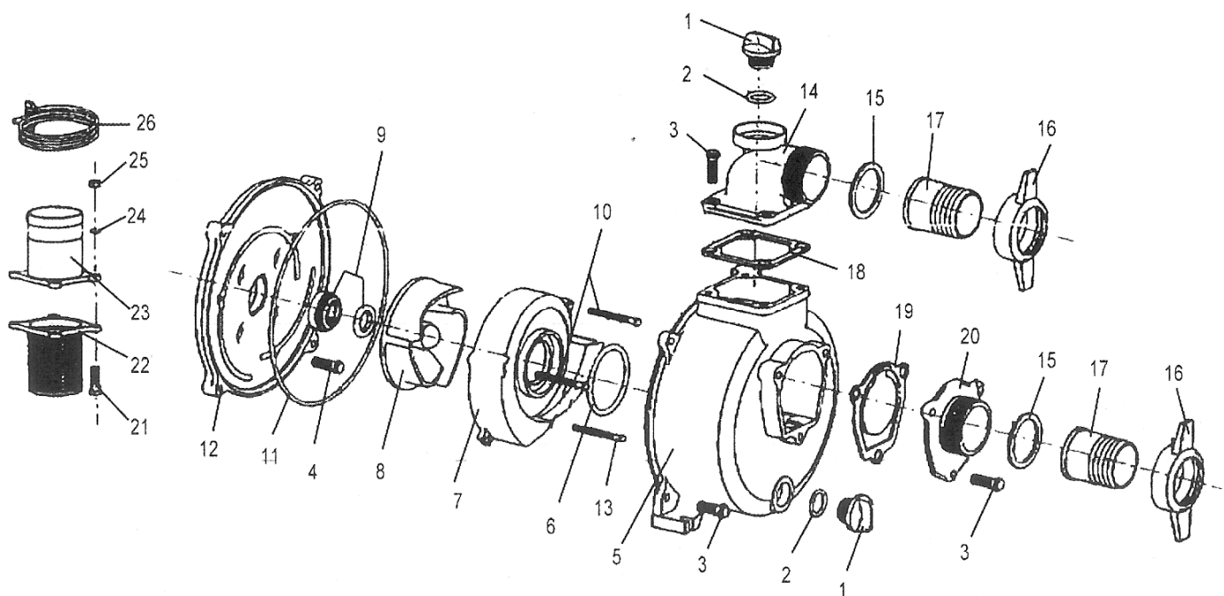
3" DIESEL PUMP
